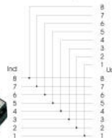
Paralleladapter
