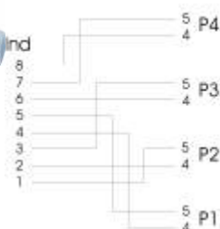
Tele adapter 1-4, T568B
