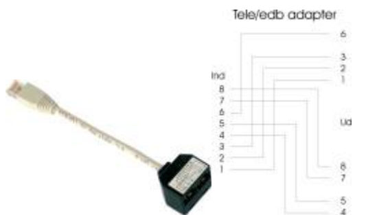
Tele/edb adapter
